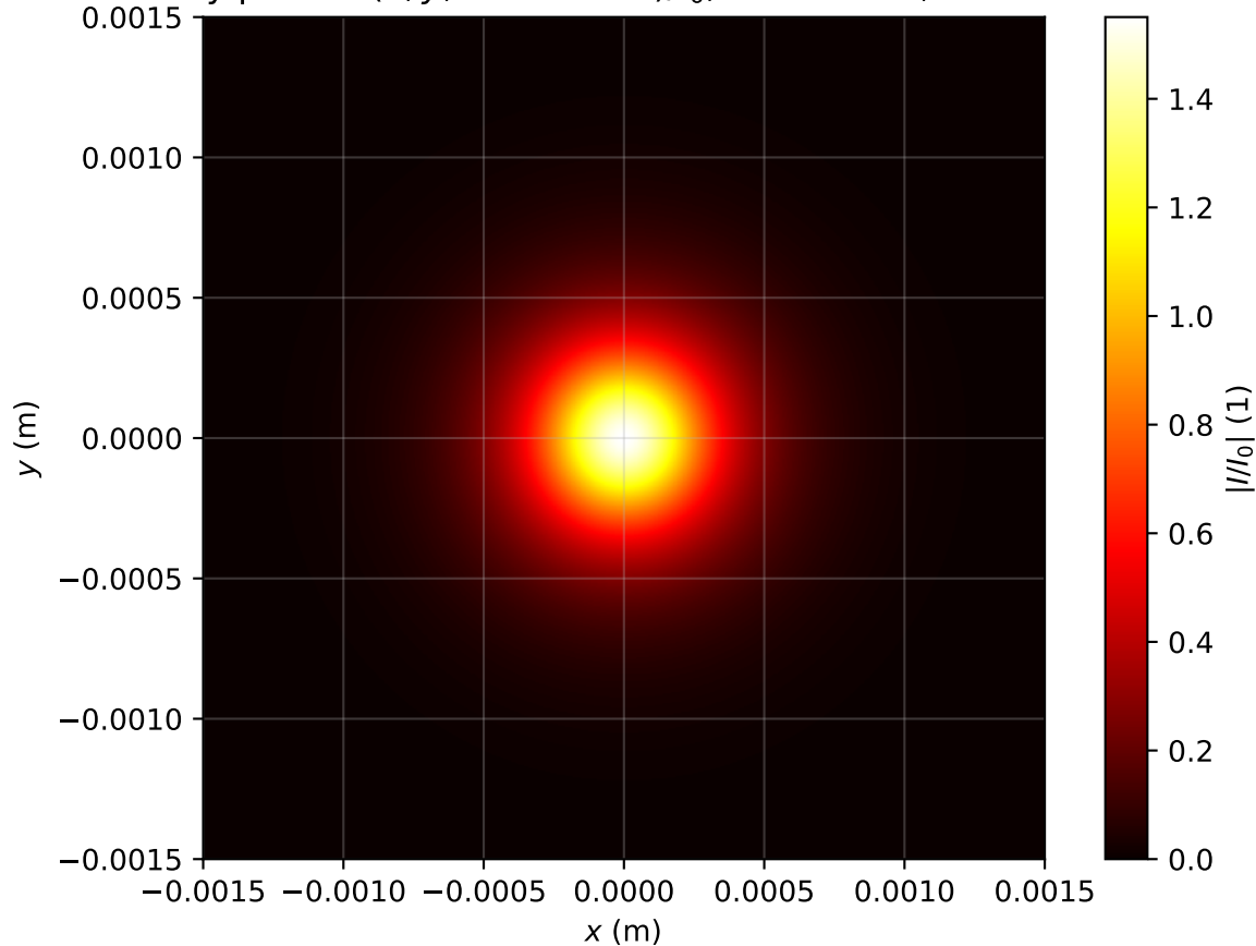
Intensity profile I(x, y, z = 1.035m)/I_0 , Pin=1.0Pcr, artificial time
